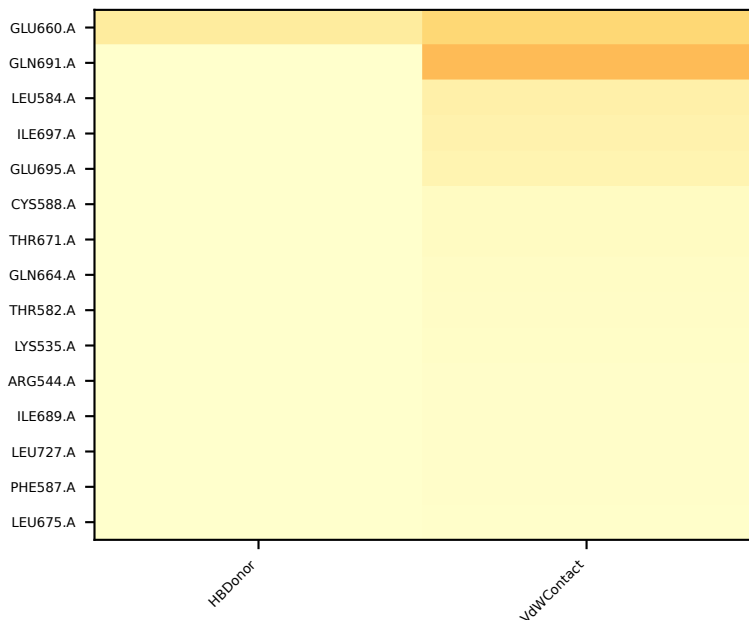
C: BMS-986205 / WT (Success)
